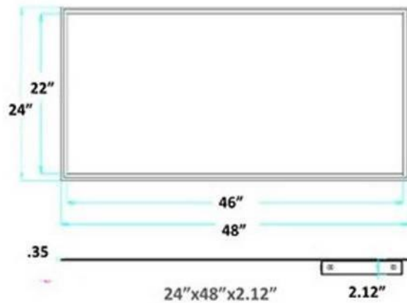
Panel light Dimension (unit: in)
