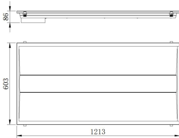
Panel light Dimension (unit: mm)
