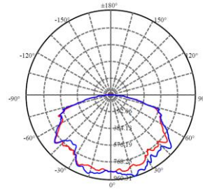
Light Distribution
