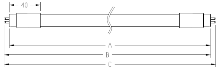
T5 tube Dimension Diagram (unit: mm)
