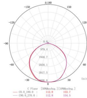
Light Distribution
